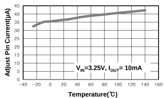
Adjust Pin Current vs. Temperature
