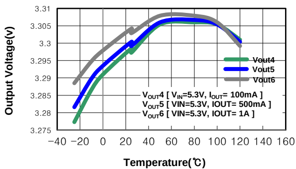
Graph 5 Electrical Characteristics Curves
